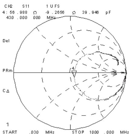
Smith chart
