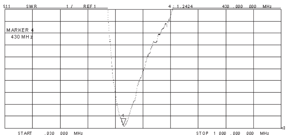
SWR characteristics
