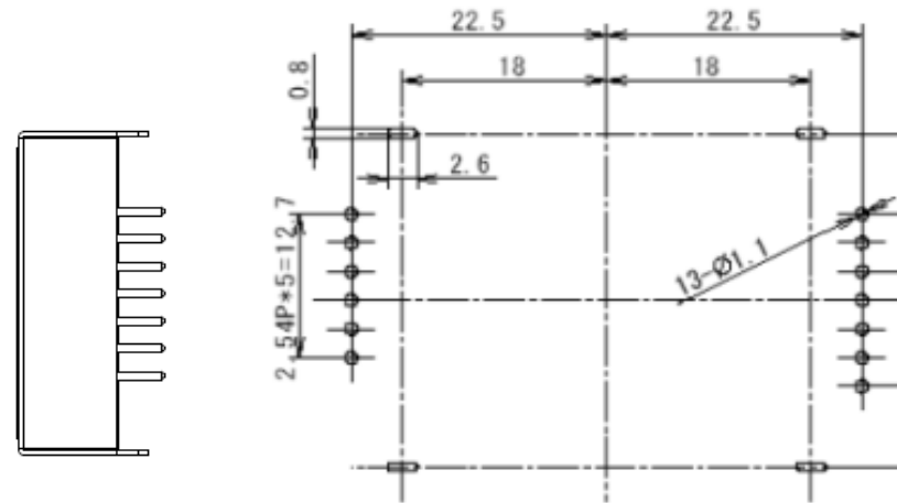
Reference hole position for PCB mounting (Top view)
