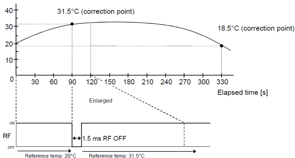
Example of RF power correction during continuous transmission
