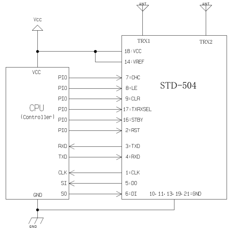
Using a common VCC voltage for the CPU and the STD-504
