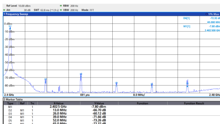
Fig.1 13MHz-spaced spurious when the channel is set to CH00
