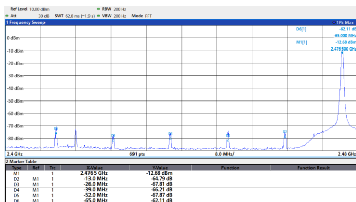
Fig. 2 13MHz-spaced spurious when the channel is set to CH4A
