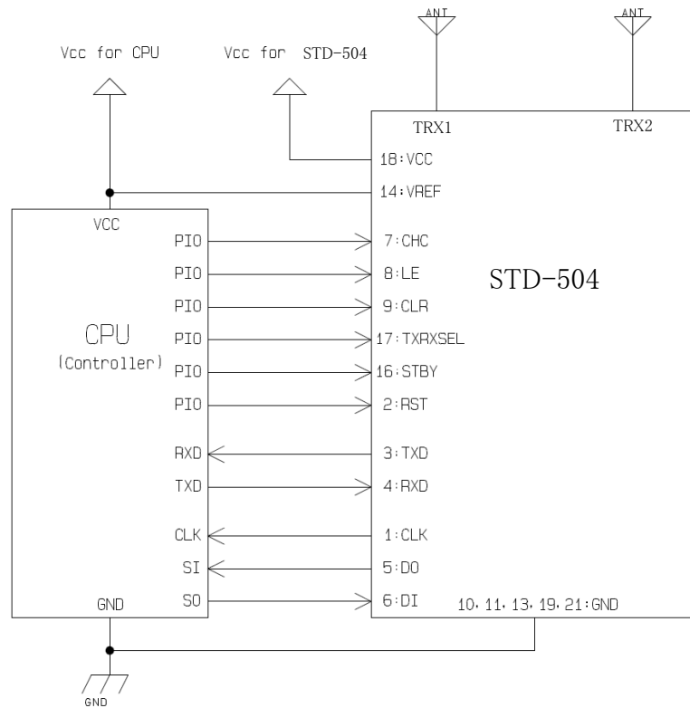
Using a different VCC voltage for the CPU and the STD-504
